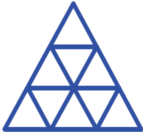
13 Triangles
